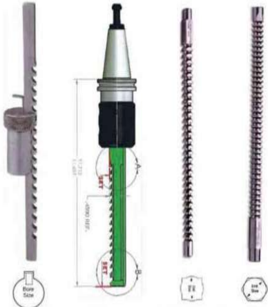
KEYWAY BROACH COLLAR SHIM
